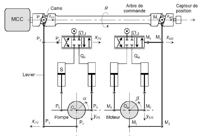
Transmission Vario
